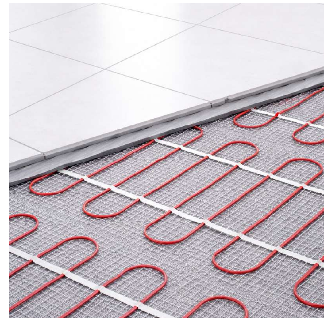
UNDERFLOOR HEATING (ELECTRIC)*
